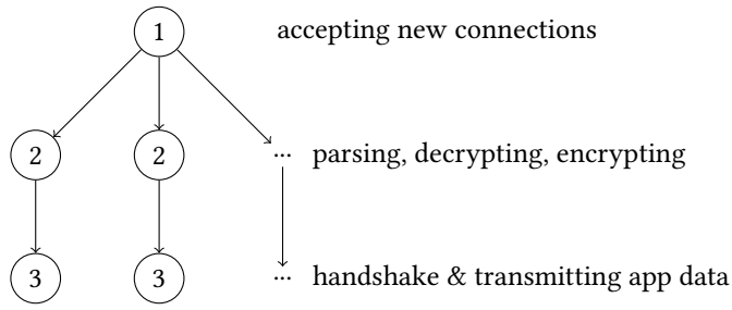
Fig. 9. Overview of our TLS implementation
